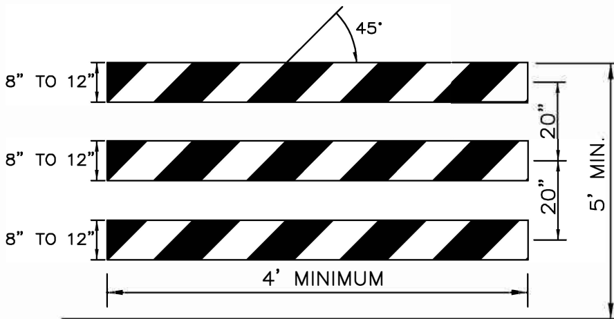
VERTICAL PANEL
