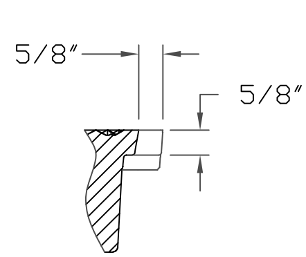
PICKHOLE DETAIL
