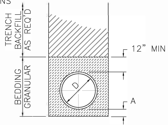
TYPICAL PIPE BEDDING
