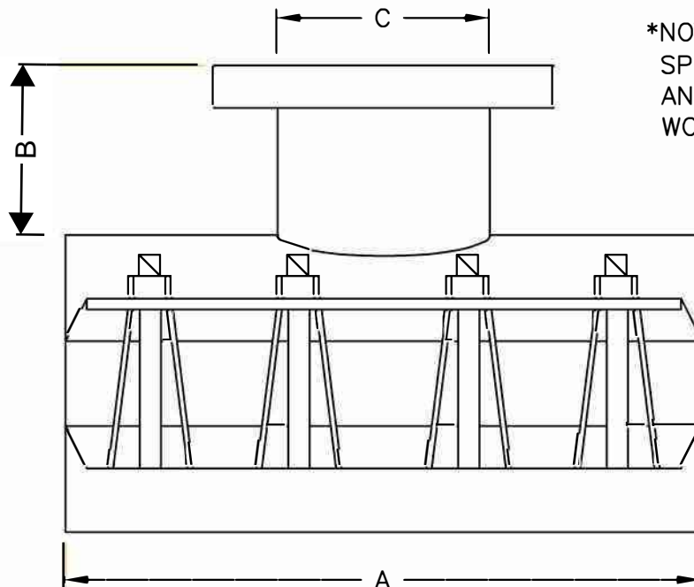
SECTION
