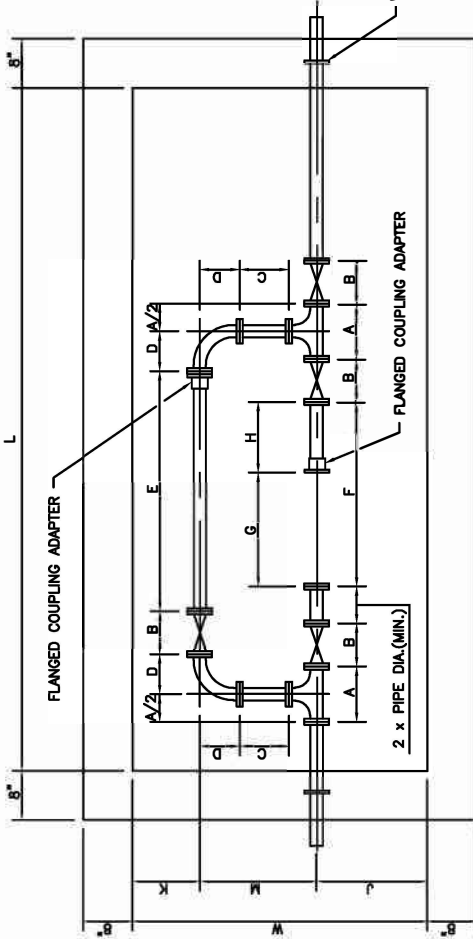
PLAN
