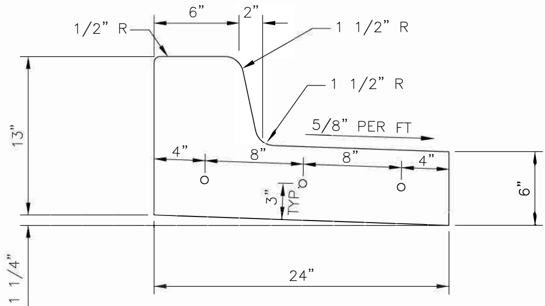
CROSS SECTION
