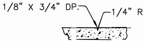
CONTRACTION JOINT
