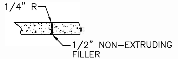
EXPANSION JOINT
