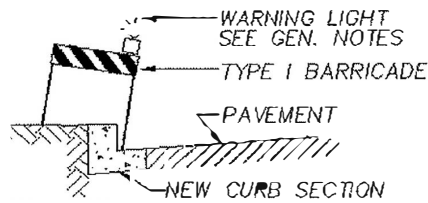
TYPICAL BARRICADE PLACEMENT DETAIL NEW CURB SECTION
